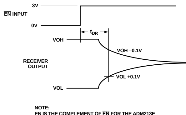
Figure 22. Receiver-Disable Timing
